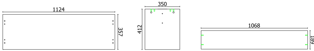
BANK ÜST PANEL 2 ADET
